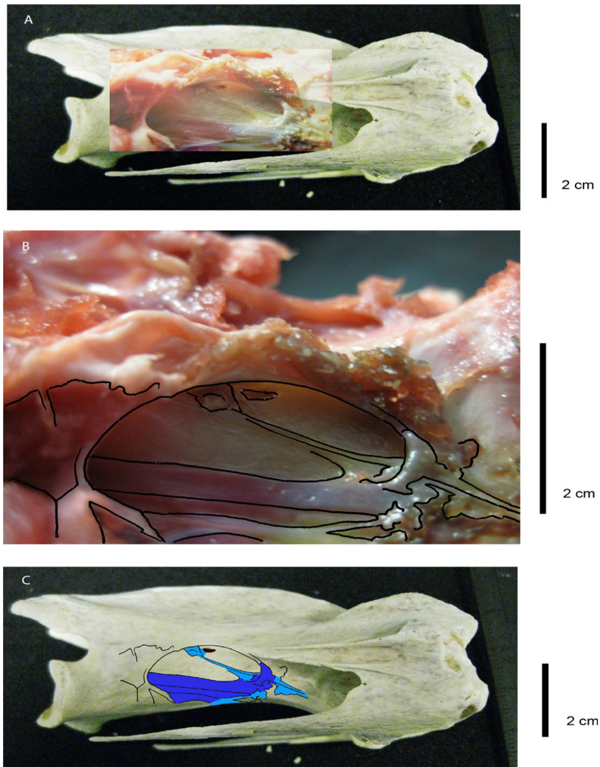
Fig 5. Triple schematic of ostrich vertebra-air sac-flesh tissue system. (A) Depiction of a semi-transparent layer of the actual close-up of the air sac diverticulum system with its surrounding tissue placed on top of the cervical vertebra; (B) Magnified air sac diverticulum and its membranous extensions. The black lines indicate the various folds and borders of the air sac diverticulum and its membranes as they expand on the bone; (C) Only the bony tissue with the schematic representation of the air sac diverticulum/membrane system without the surrounding flesh tissue. Same colour codes apply as described in Fig 2. Please note that the air sac is not inflated and thus intraspecific variation is highly probable.
