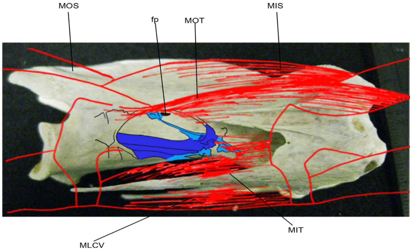
Fig 2. Schematic representation of air sac complex with its associated muscles. Right lateral view of a Struthio camelus (ostrich) mid-cervical vertebra, showing a local fraction of the air sac diverticular complex and the muscle groups (red) associated with it and the vertebra. The black lines represent the various borders of the diverticular membrane extensions; the purple shows the air sac's lateral vertebral diverticulum along the corpus; the light blue depicts the membranes that extend from the diverticulum, anchoring on the corpus and invading the brown foramen pneumaticum. Abbreviations: fp foramen pneumaticum; MOS M. obliquospinalis ; MOT M. obliquotransversalis ; MIS M. interspinalis ; MLCV M. longus colli ventralis ; MIT M. intertransversalis .
